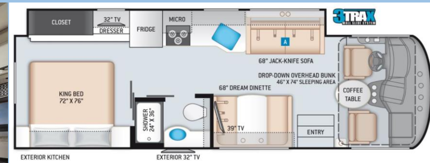
Floorplan ACE 29.3
